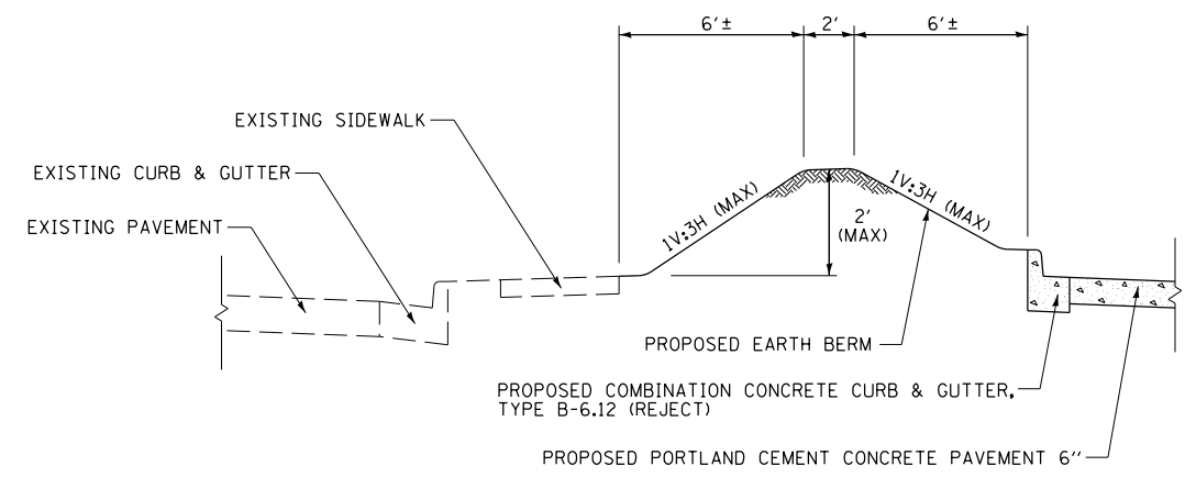
SECTION A-A PROPOSED BERM DETAIL
